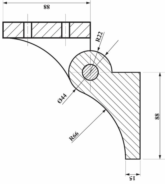
SECTIONAL ELEVATION A - A
